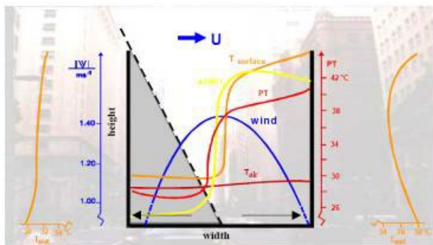
Cross section of street canyon. PT and micro-scale input variables.
